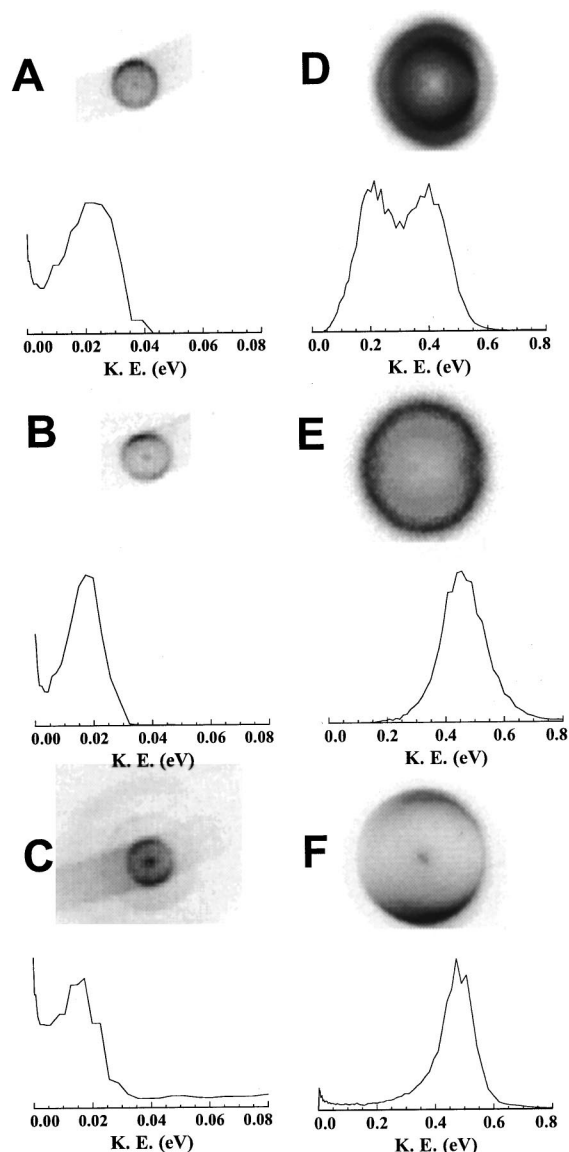
FIG. 2. Photoelectron images and electron kinetic energy release distributions for several resonant lines of O_4^+ . Wavelengths are (a) 323.478 nm, (B) 306.122 nm, (C) 304.987 nm, (D) 296.788 nm, (E) 294.893 nm, and (F) 282.836 nm.
