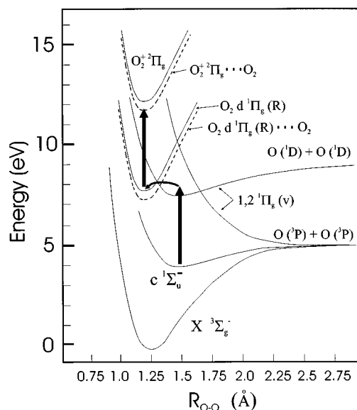
FIG. 3. Relevant potential curves adapted from Ref. 23, from calculations of Ref. 21. The Rydberg and ion curves, duplicated and offset -0.45 eV (the energy of the O_2-O_2^+ bond) are shown as dashed lines (see the text).
