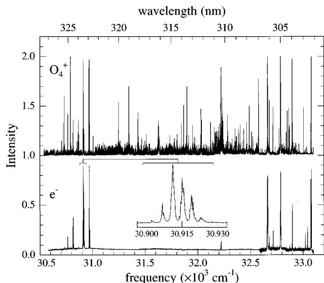
FIG. 1. Raw O_4^+ photoion yield and total photoelectron yield spectra. Expanded region of the electron spectrum is shown in the inset.
