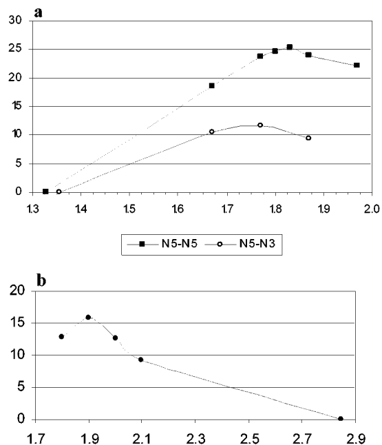
Figure 4. Electronic Energy (kcal/mol) with respect to 1 or 2 from partial optimizations at RI-MP2-fc/TZVPP. (a) Energy of 1* and 2* as a function of the N2–N3 distance. (b) Energy of 1* as a function of the N5–N10 distance.
